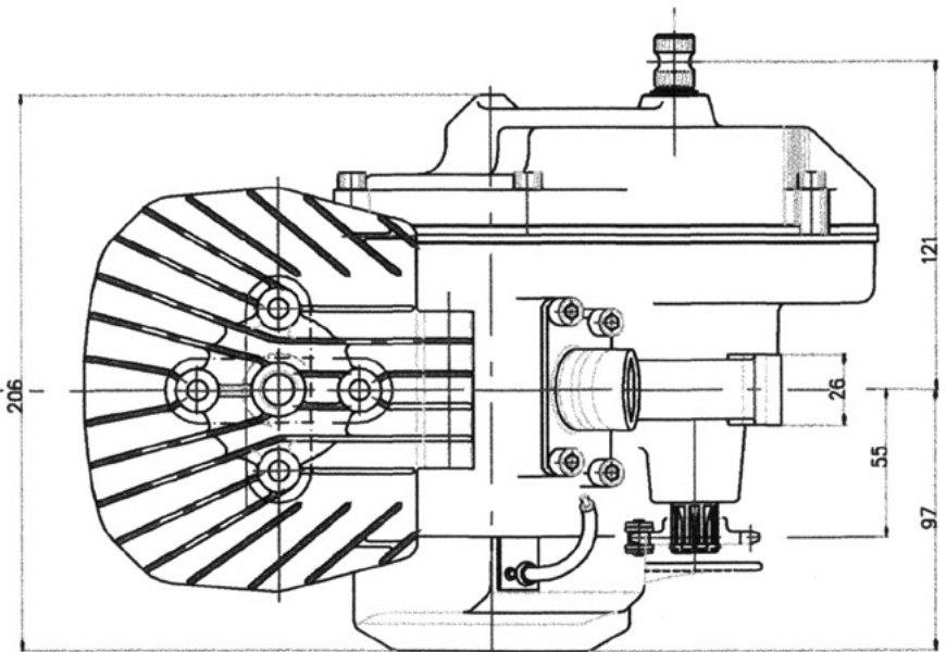
FRONT FRAME CONNECTION (Attacco anteriore)
